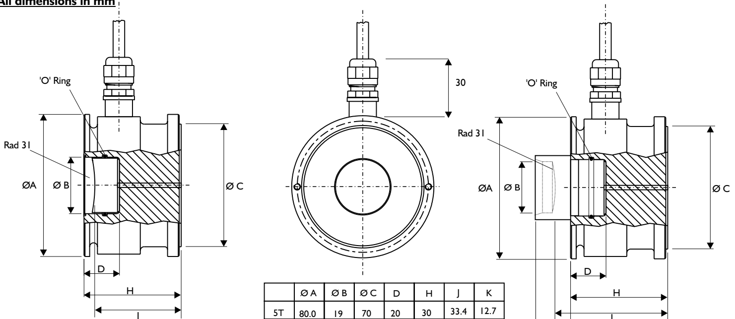
20-50 Tonne Capacity
